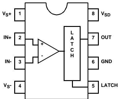
EL5185 (8-PIN SO) TOP VIEW
